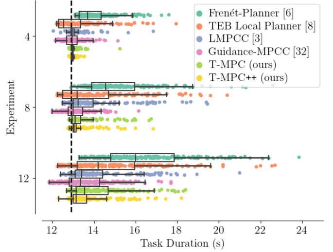
Fig. 7. Visualization of the task duration (i.e., the time taken to reach the goal) in Table II. The dashed vertical line denotes the task duration without obstacles. Our method achieves the smallest variation in task duration and the shortest task duration in crowded environments.
