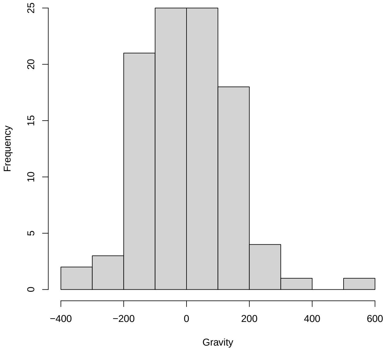
Histogram of Gravity
