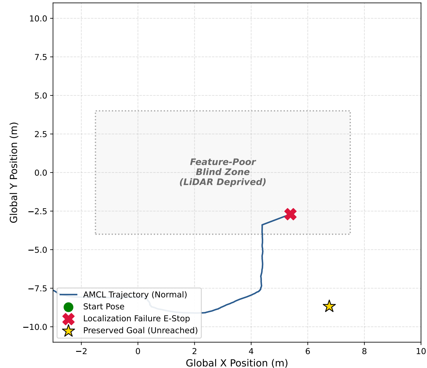
(a) Baseline Conventional System (Stranded at Feature-Poor Zone)
