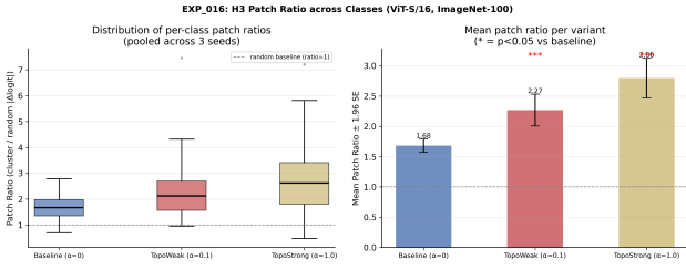
Figure 2. H3: Causal patching ratios across 20 classes \times 3 seeds ( n = 60 ). Each point is the mean cluster/random logit-delta ratio for one class \times seed combination. The ratio at \alpha = 1.0 ( 2.79 \pm 1.24 ) is significantly above baseline ( 1.68 \pm 0.42 ), and above \alpha = 0.1 ( 2.27 \pm 0.93 ). Both comparisons: p < 0.0001 , Cohen’s d \geq 0.61 . Per-seed means at \alpha = 1.0 : 2.53, 2.89, 2.97 — no outlier drives the effect.
