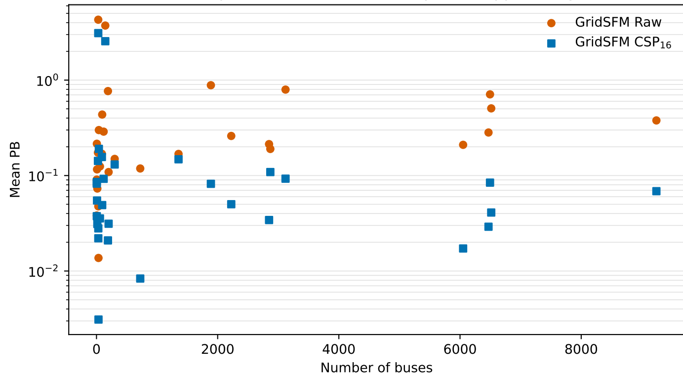
GridSFM power-balance consistency across ppNR-v2 grids
