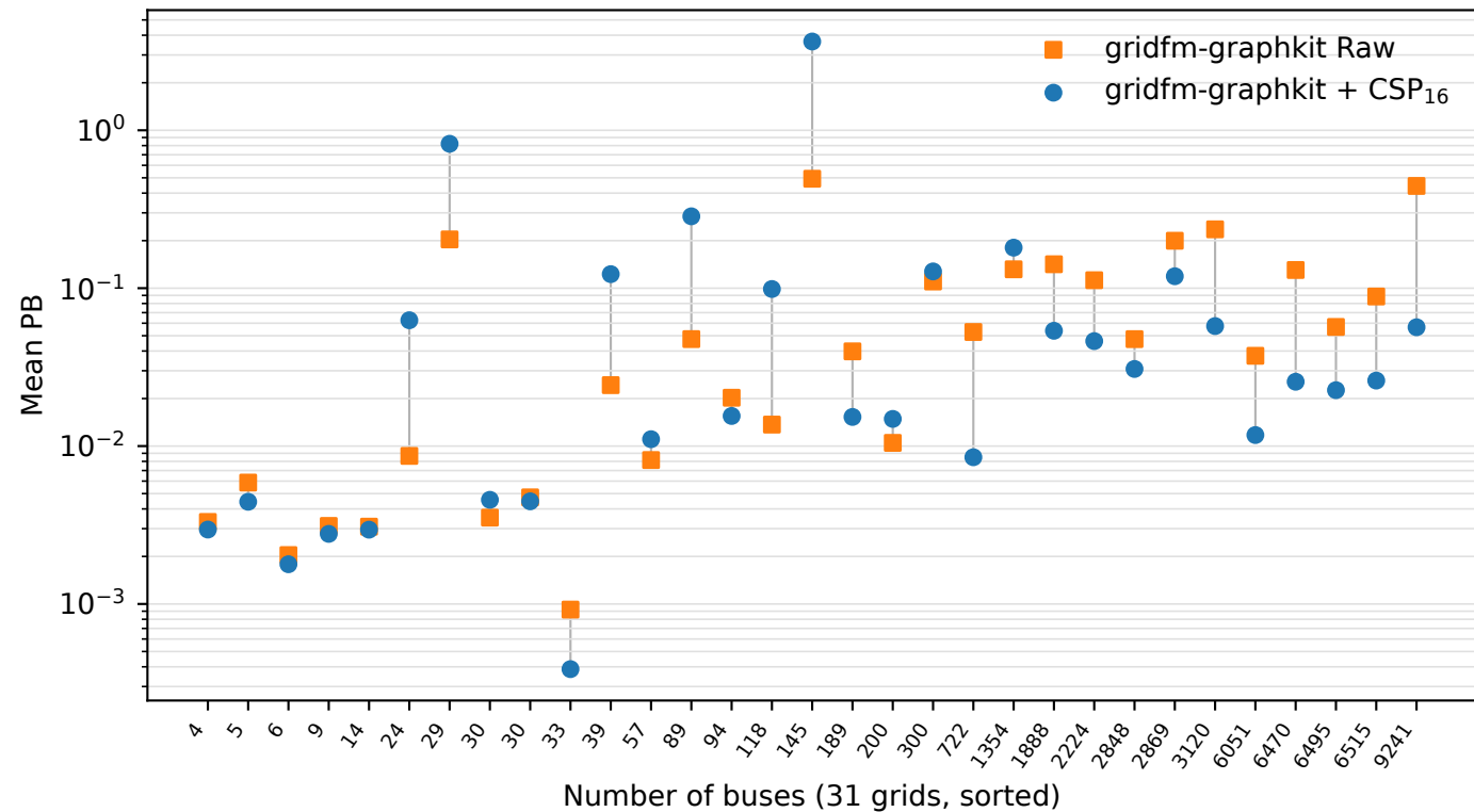
gridfm-graphkit power-balance consistency across 31 grids
