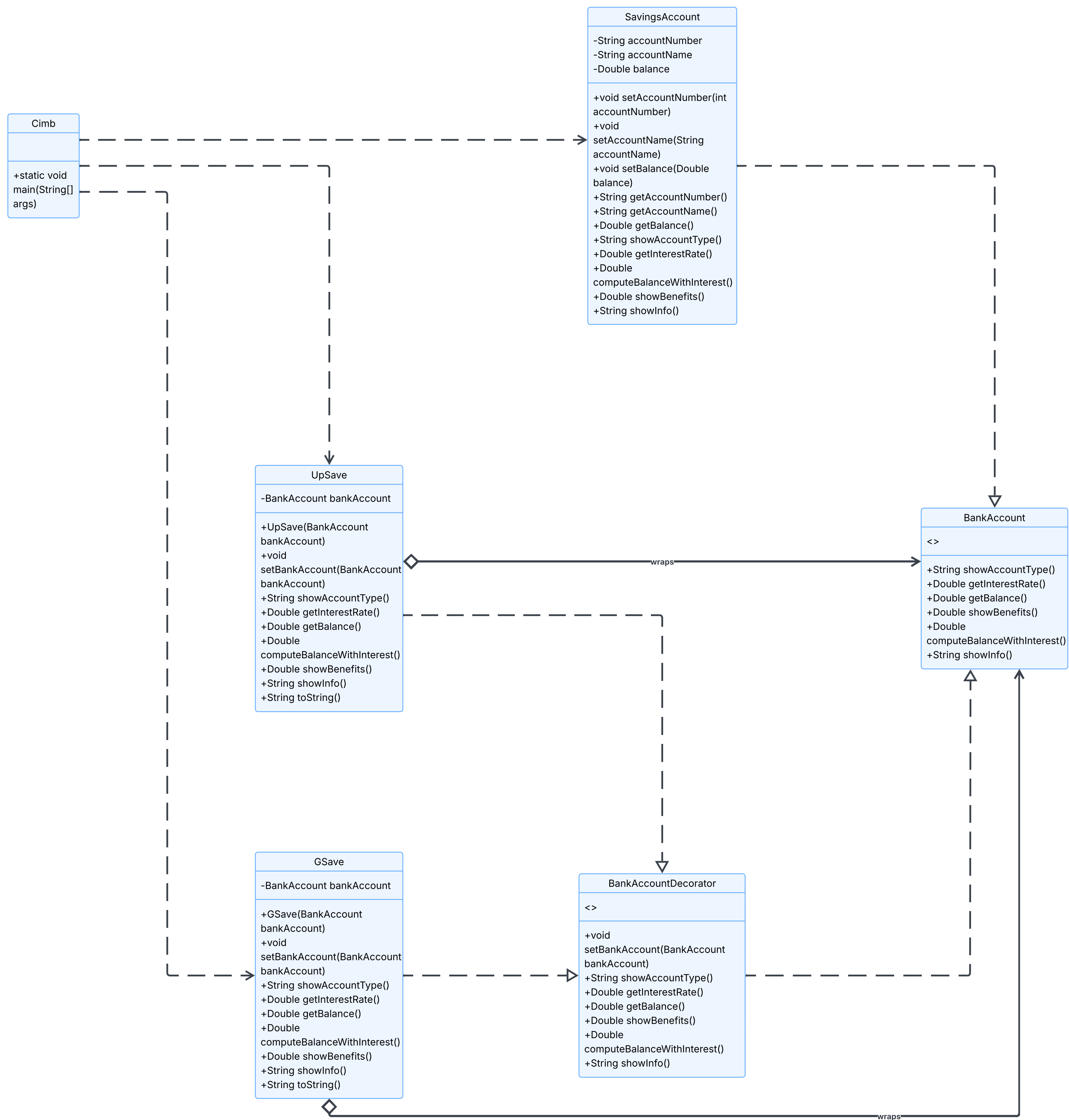
UML Class Diagram for BankAccount System
