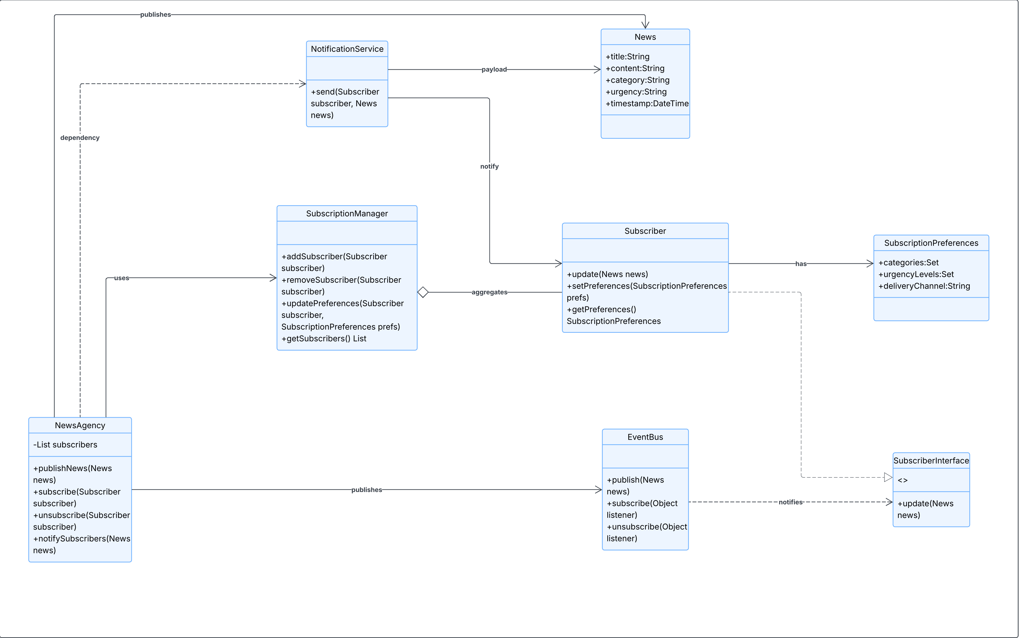
Real-time News Subscription UML Diagram
