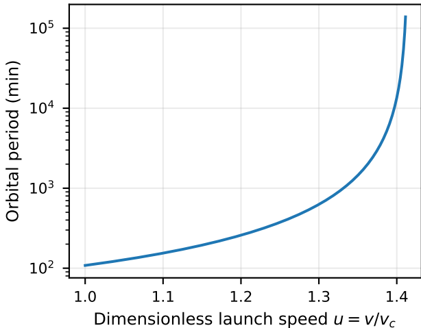
Period diverges near escape
