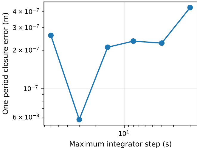
Numerical convergence against the analytic orbit
