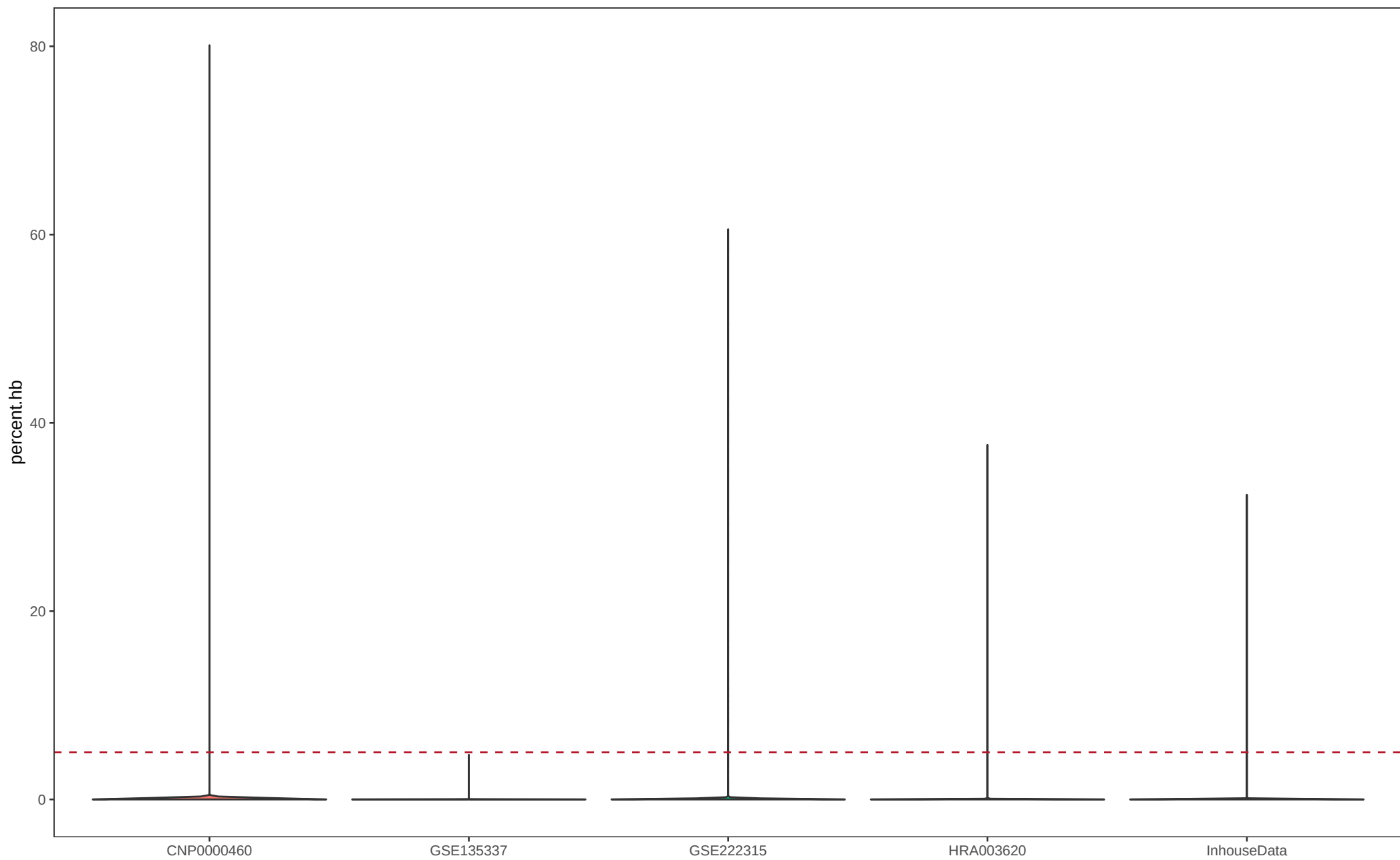
percent.hb by dataset
