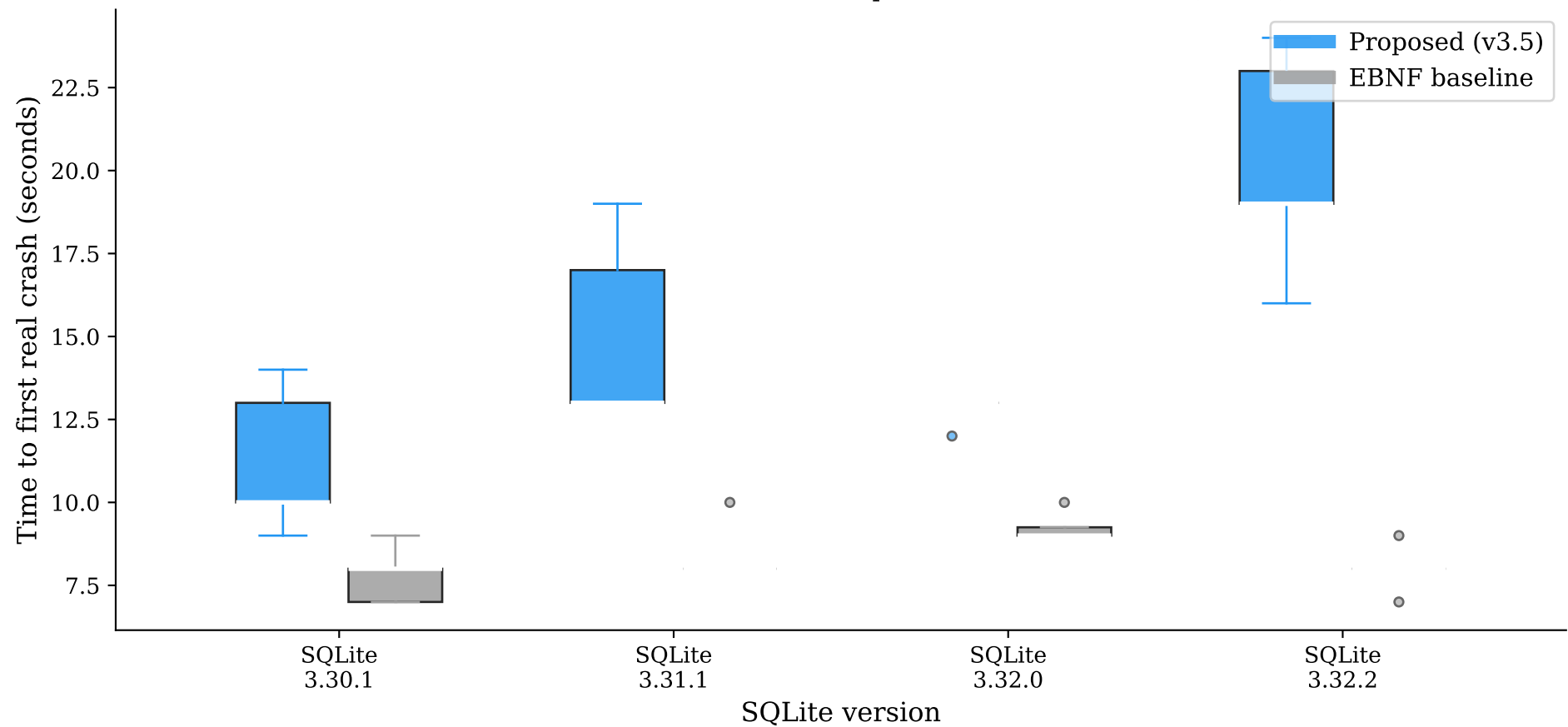
Time to First UBSan/ASan Crash - Proposed vs. EBNF Baseline (5 runs)
