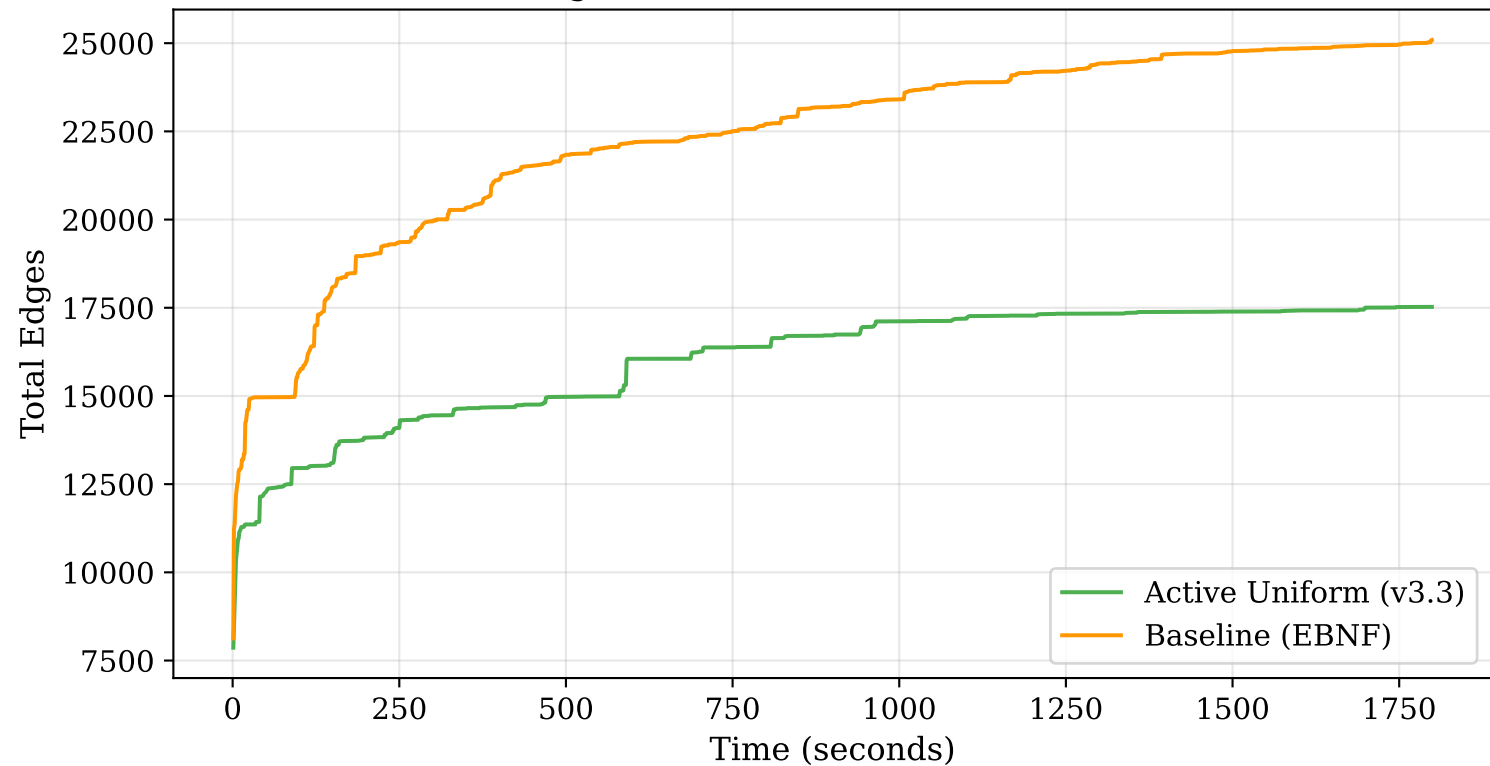
Coverage Growth — SQLite 3.31.1 (30 min)
