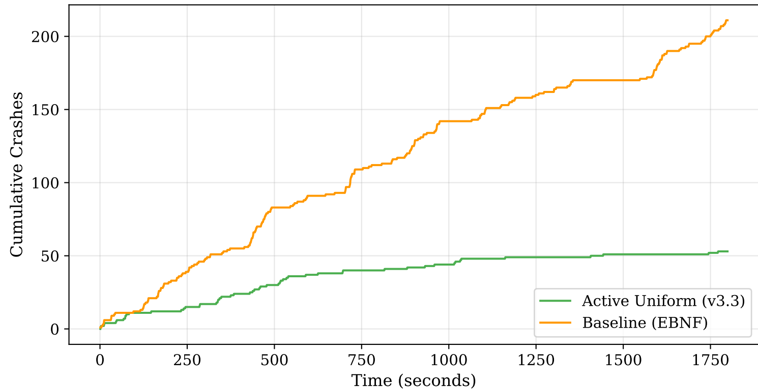
Crash Accumulation — SQLite 3.31.1 (30 min)
