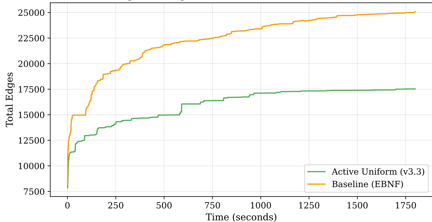
Edge Coverage Growth — SQLite 3.31.1 (30 min)
