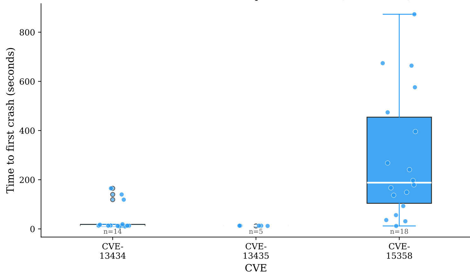
Time to First CVE Crash - Proposed Grammar (v3.5, 15 min)
