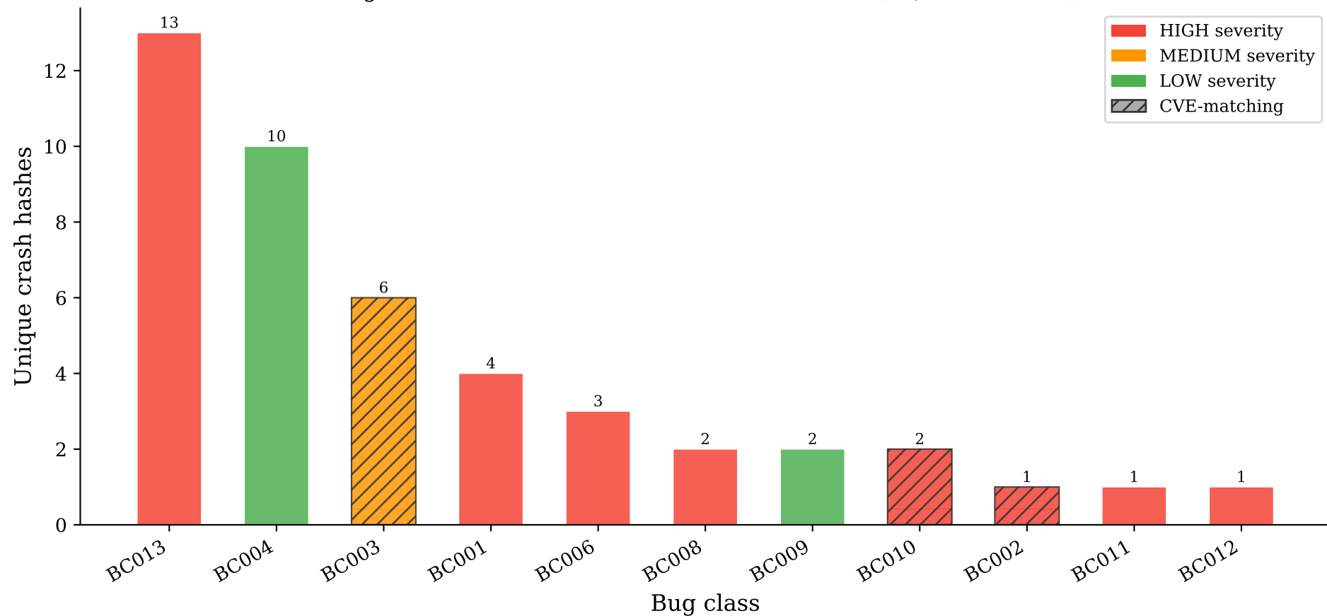
Bug Class Breakdown - Unseen Grammar v3.3 (RQ2, 4 × 5 runs)
