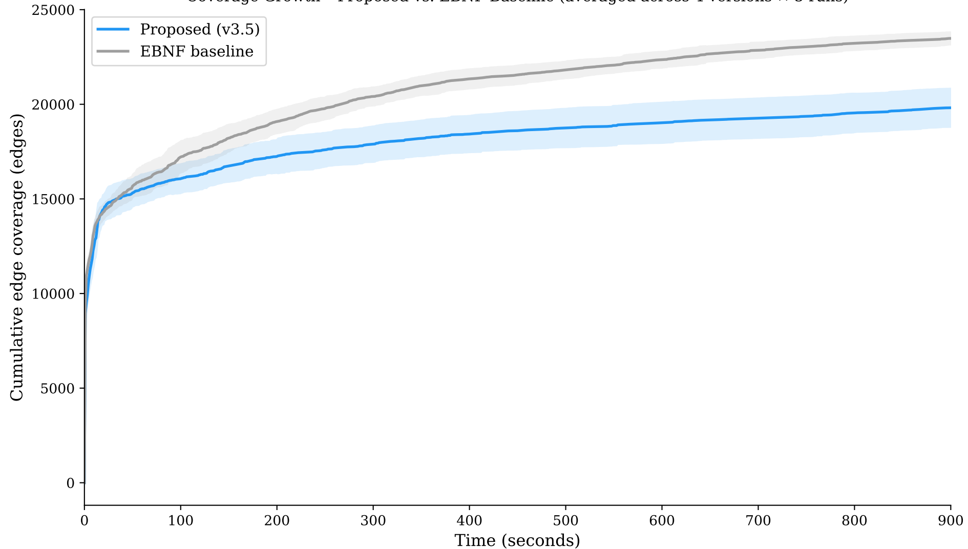
Coverage Growth – Proposed vs. EBNF Baseline (averaged across 4 versions \times 5 runs)
