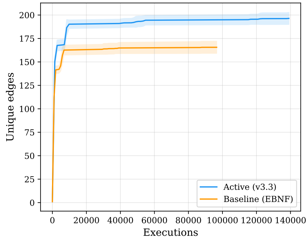
SQLite 3.31.1
