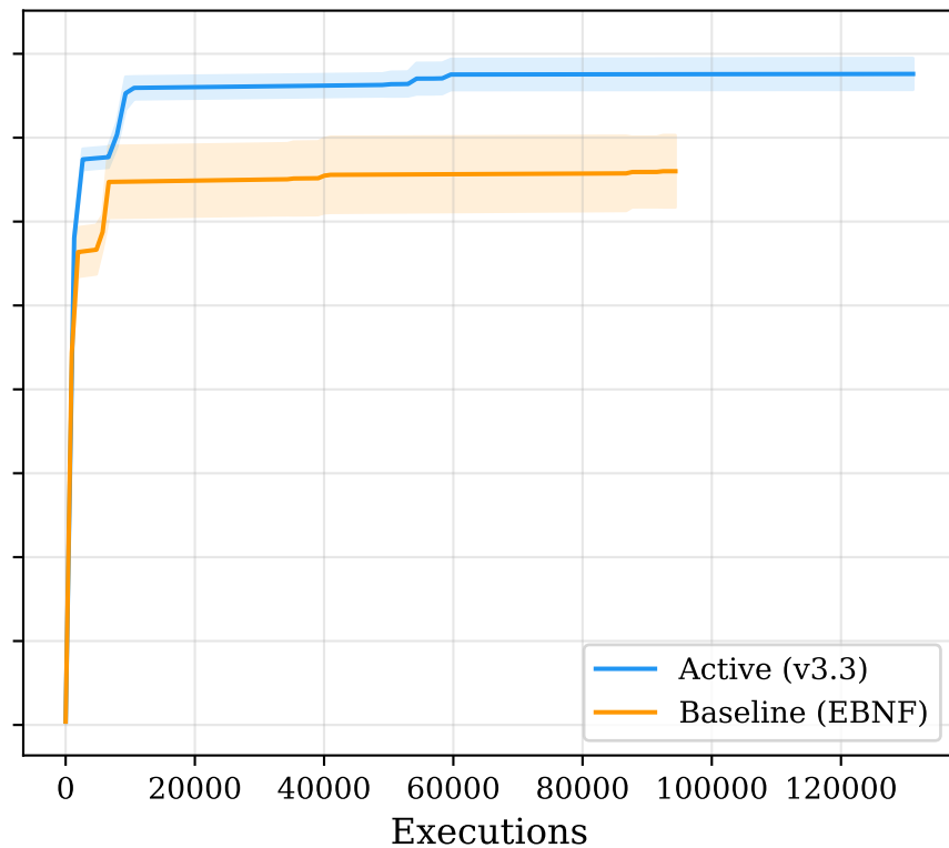
SQLite 3.32.2
