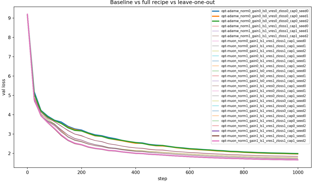
Figure 1: Validation-loss curves for the anchor configurations (all-off AdamW baseline and all-on full Muon recipe, bold) and the leave-one-out runs (full recipe with one toggle removed). The full-recipe band separates cleanly from the baseline early and holds the gap for the rest of training; the highest leave-one-out trajectory is the one dropping QK-norm.
