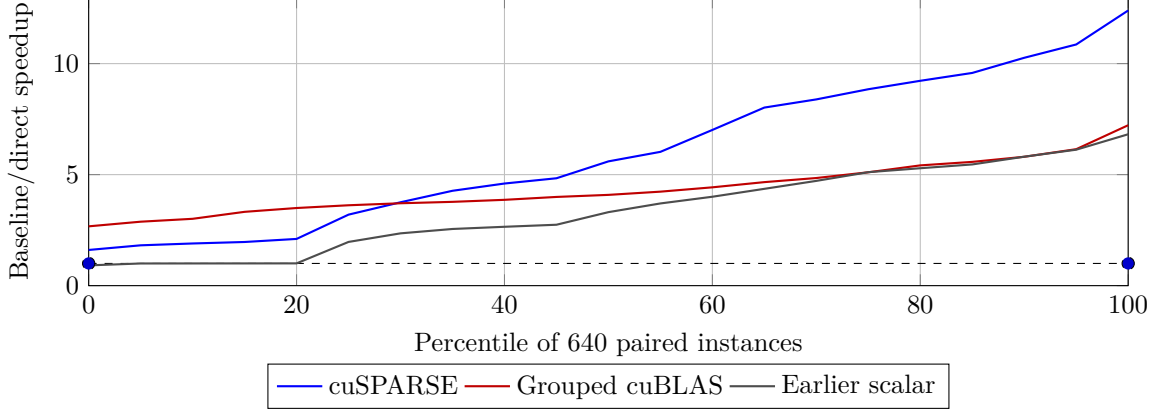
Figure 1: Empirical speedup distributions over all 640 paired workload–seed instances, plotted at five-percentile increments. The dashed line denotes parity; both library distributions remain above it, while the earlier scalar kernel has near-parity RHS-8 cases.
