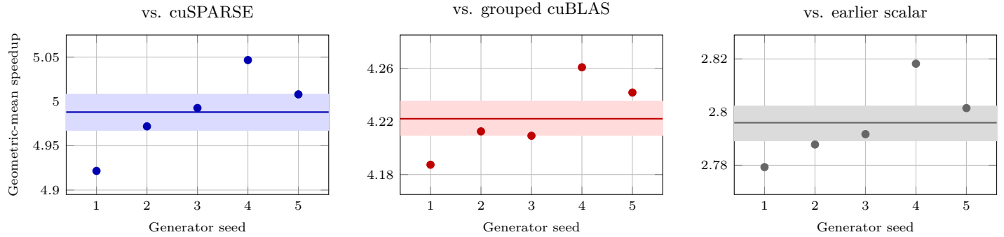
Figure 2: Repeated-seed replication error. Markers are the per-replicate geometric-mean speedups from Table 2, each obtained by running the complete 128-configuration grid under one generator seed. The solid line is the across-replicate mean and the shaded band is that mean plus and minus one standard error. Note the suppressed zero and the narrow, panel-specific vertical ranges: all five replicates of every comparator fall within about 1% of their mean, so the replication error is far smaller than any of the reported effects.
