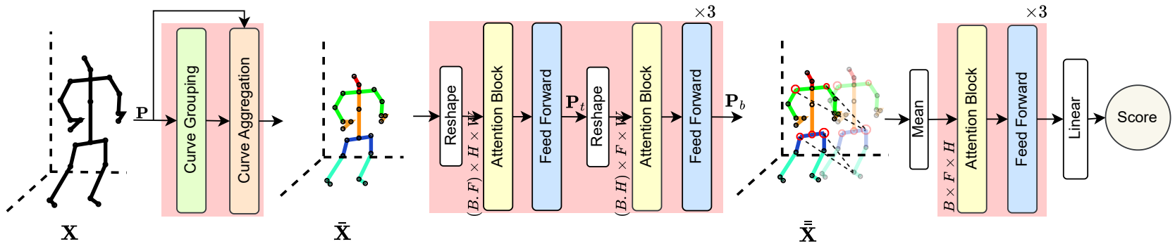
1. Overall Architecture of the Attention Based Transformer Model
