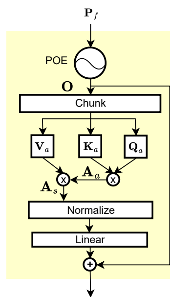
1. Overall Architecture of the Attention Based Transformer Model
