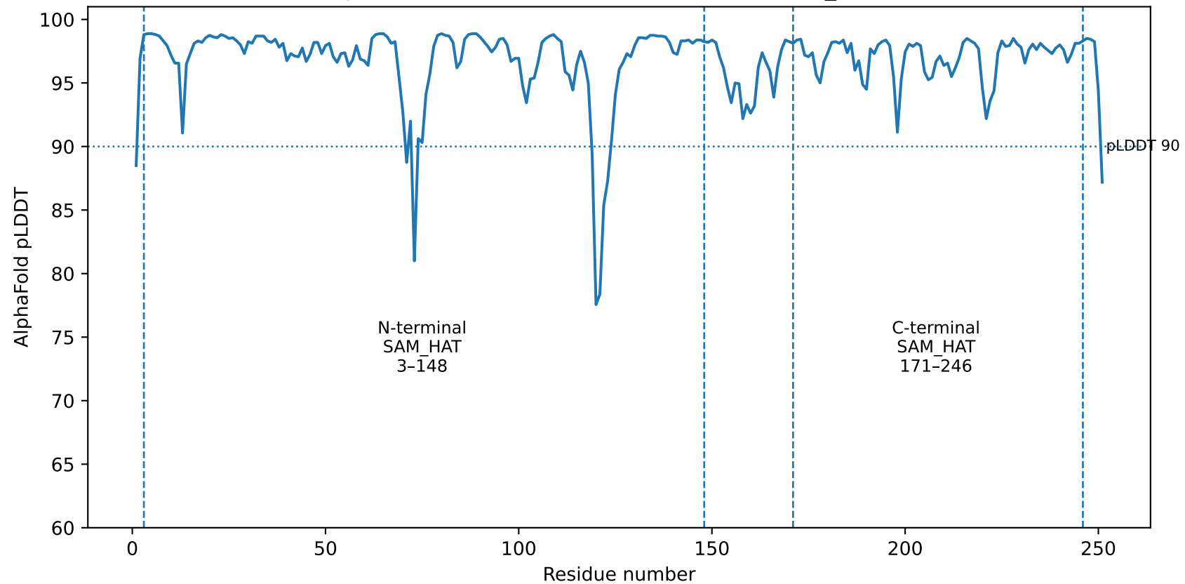
AlphaFoldDB v6 local confidence for O67940_AQUAE
