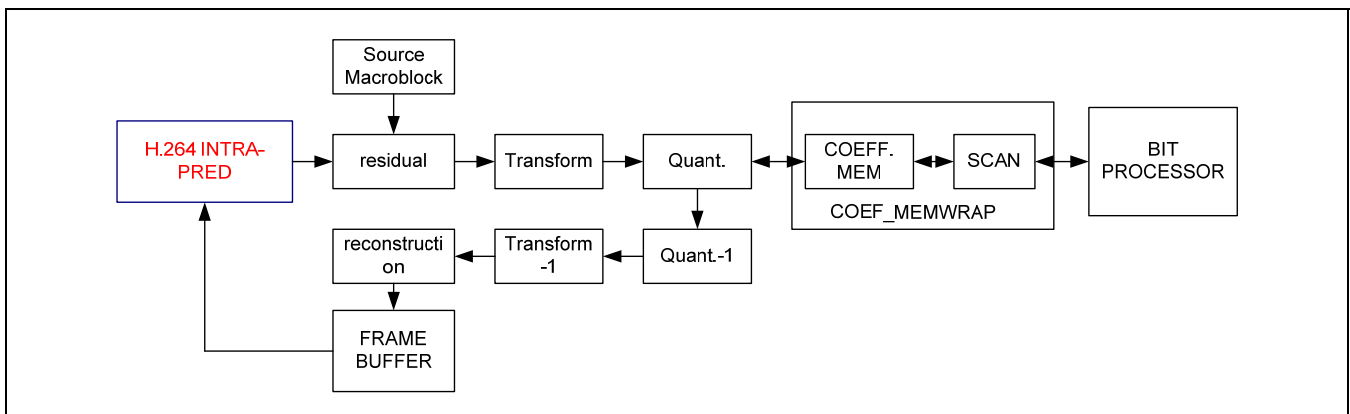
Figure 21-17 (b). H.264 Intra prediction data flow
