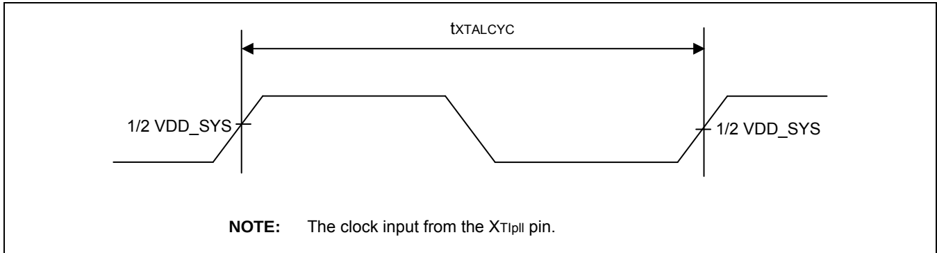
Figure 44-1. XTlpII Clock Timing
