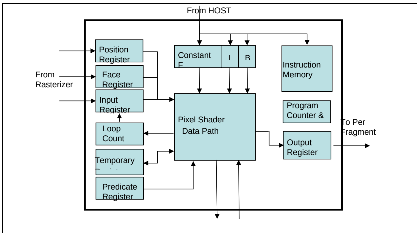
Figure 6-1 Pixel Shader Block Diagram
