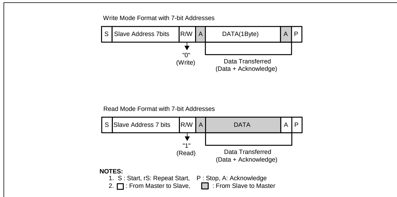
Figure 30-3. Data Transfer on the IIC-Bus Block Diagram
