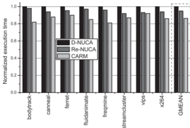
Fig. 10. Execution time normalized to D-NUCA.
