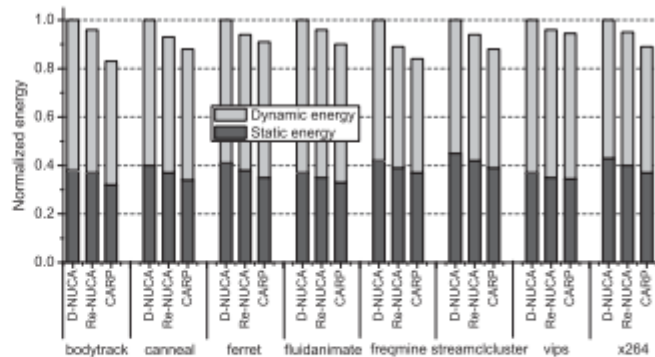
Fig. 11. Energy normalized to D-NUCA.
