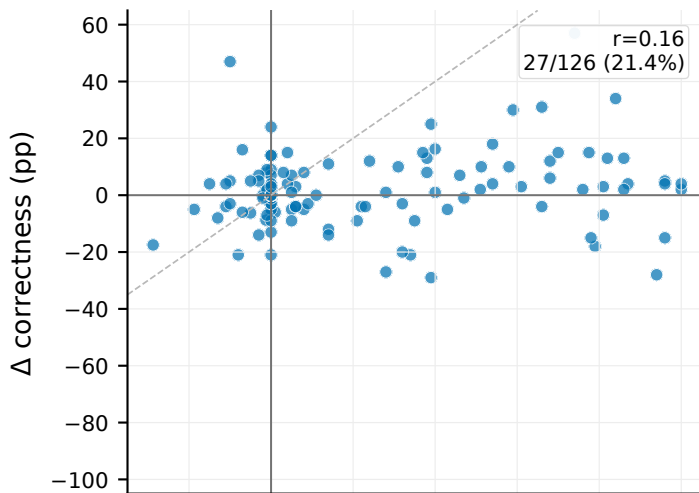
MBPP
