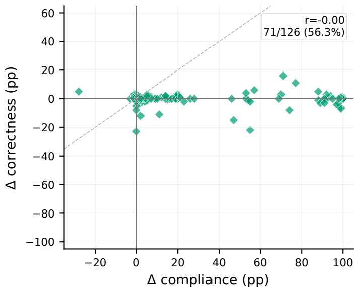
MBPP
