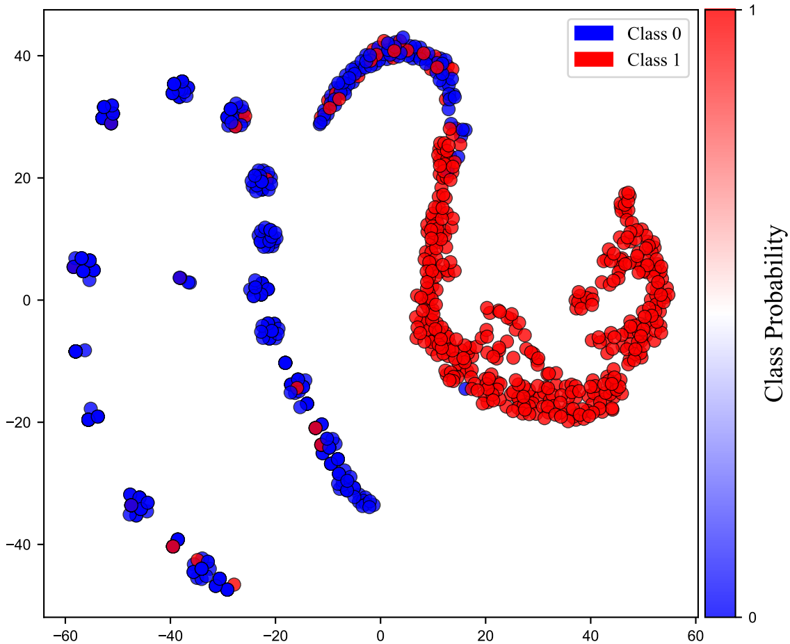
t-SNE Visualization
