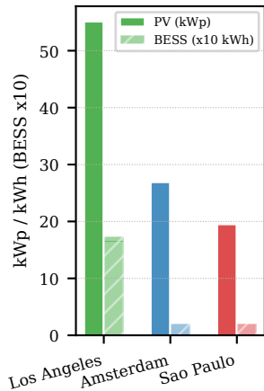
(b) PV and BESS sizing
