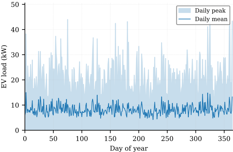
(a) Annual EV load profile, JPL Arroyo Garage
