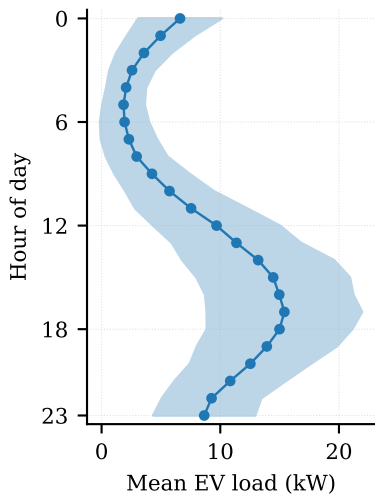
(b) Diurnal profile
