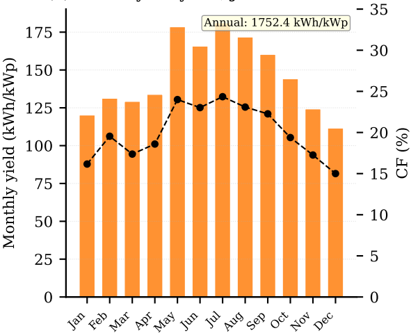
(a) Monthly PV yield, JPL Pasadena CA
