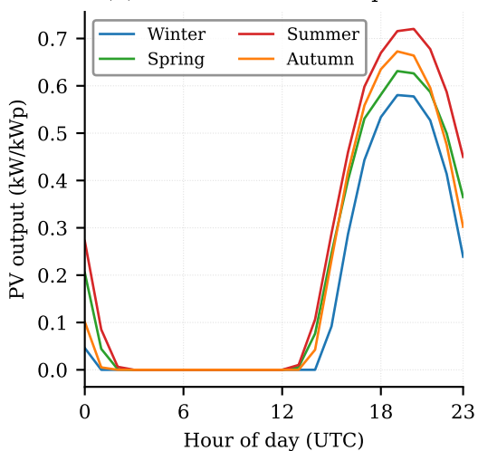
(b) Seasonal diurnal PV profile
