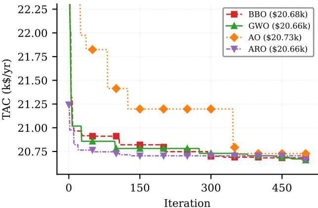
Convergence: Case 4 PV+BESS+SC+Grid
