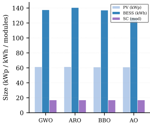
(b) Optimal sizing: Case 4
