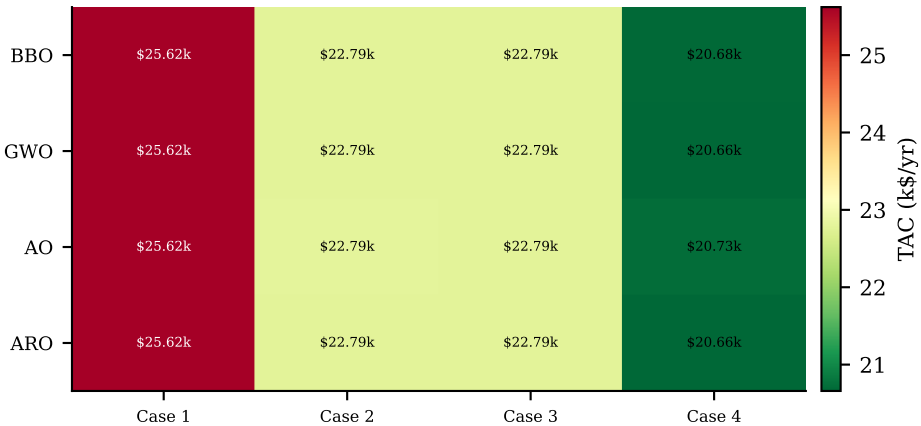
TAC (k$/yr) by algorithm and case
