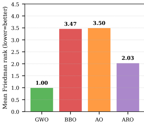
(b) Friedman mean rank ( \chi^2 = 79.24 , p = 0.0000 )
