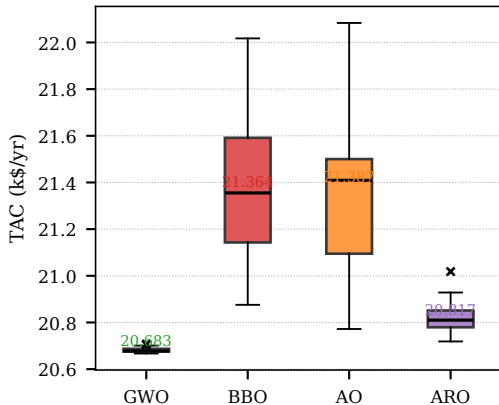
(a) TAC distribution (30 independent runs)
