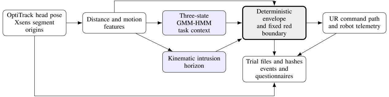
Fig. 1. Prototype architecture. In SSM mode, learned outputs can add caution but cannot raise the command above the deterministic envelope. Logging spans sensing, decisions, commands, and measured robot response. The software bound is not a certified safety function.
