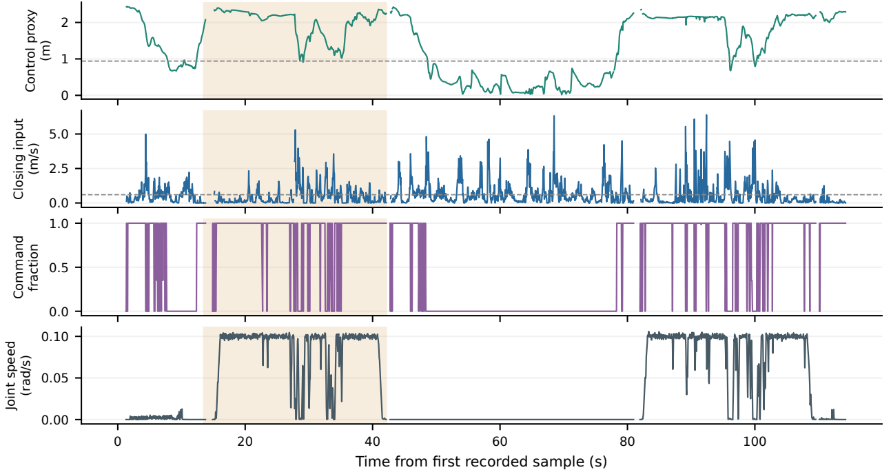
Fig. 4. P24 T01: recorded body-proxy distance, closing input, command fraction and maximum absolute fresh joint velocity. Shading marks the dashboard event window. Dashed lines are configuration thresholds. Gaps over 250 ms break the lines. The plot is an observed trace, not a counterfactual controller comparison.
