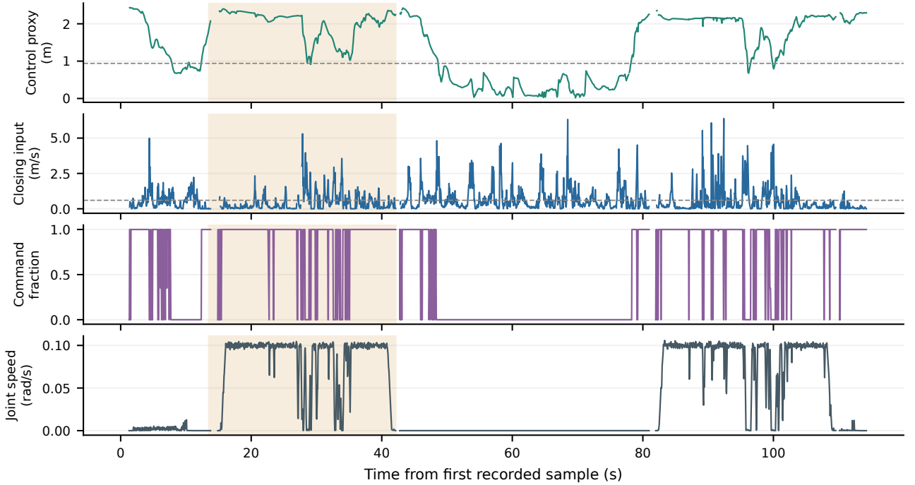
Fig. 3. P24 T01: recorded body-proxy distance, closing input, command fraction and maximum absolute fresh joint velocity. Shading marks the dashboard event window. Dashed lines are configuration thresholds. Gaps over 250 ms break the lines. The plot is an observed trace, not a counterfactual controller comparison.
