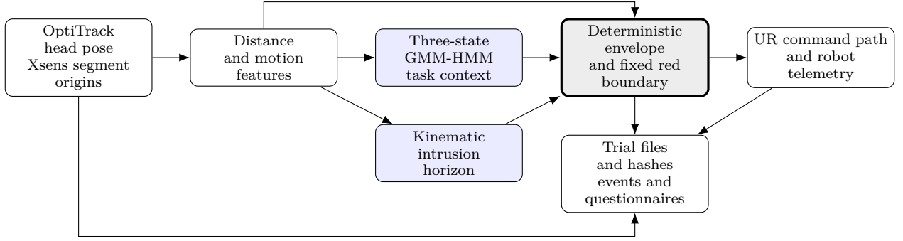
Fig. 1. Prototype architecture. In SSM mode, learned outputs can add caution but cannot raise the command above the deterministic envelope. Logging spans sensing, decisions, commands, and measured robot response. The software bound is not a certified safety function.
