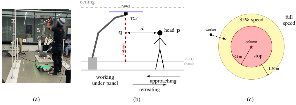
Fig. 1. The application scenario. (a) Ceiling-panel installation in our lab: the robot holds the panel at ceiling height while the worker fixes it from below (frame from session video; face blurred). (b) Side view (schematic): the worker approaches, works under the panel and retreats; the robot is represented by a vertical column under the tool centre point (TCP), and d is measured from the head p to the nearest column point q (later system version). (c) Plan view, radii to scale: the fixed controller's zones around the column and the speed allowed in each.
