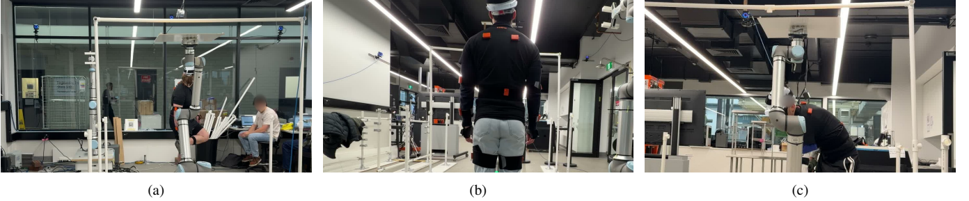
Fig. 3. Lab equipment. (a) The cell: the UR10 arm holding the panel stand-in at ceiling height, OptiTrack cameras on the overhead frame, and the operator desk. (b) A participant wearing the Xsens suit and OptiTrack cap, seen from behind while walking toward the robot. (c) The working phase: the participant works under the raised panel. Faces are blurred.
