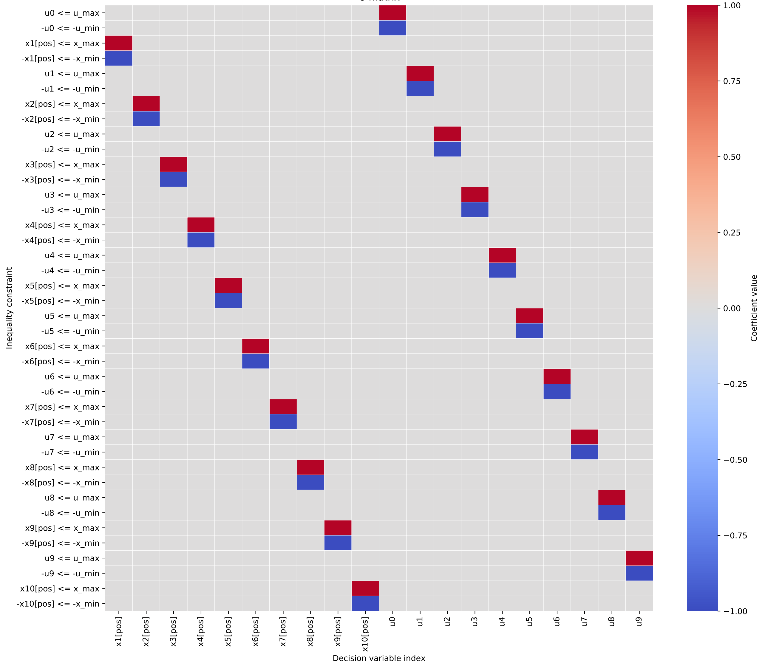
G matrix
