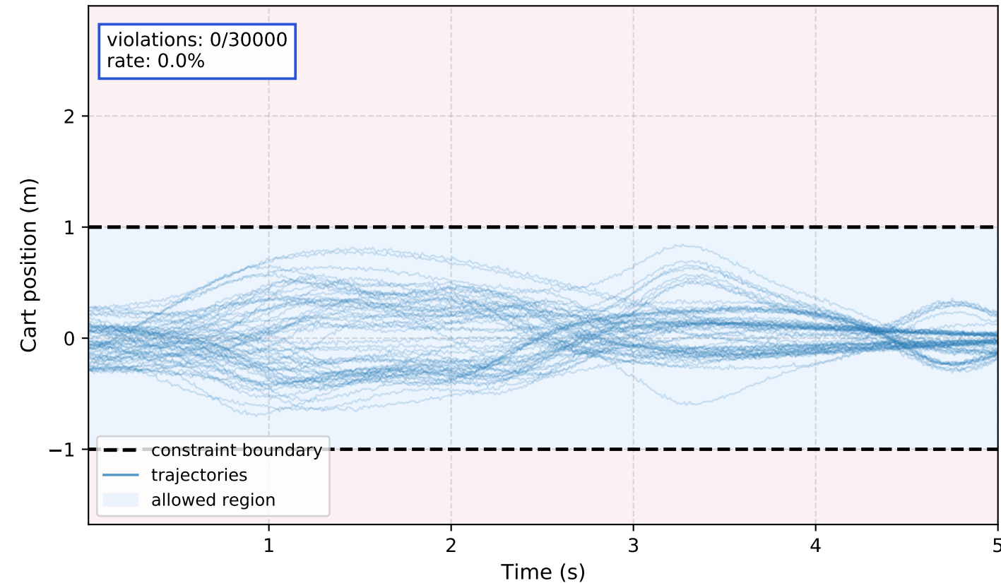
OptNet (60 trajectories)
