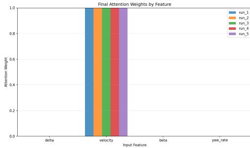
Figure 2. Final converged attention weights for each input feature from a representative experimental run (seed=42). The plot shows which features the attention mechanism deemed most important for parameter identification after training converged. This pattern of prioritizing velocity is consistent across all 5 independent experimental runs.
