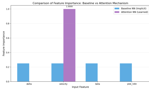
Figure 3. Comparison of feature importance between baseline neural network and attention-enhanced neural network from a representative experimental run (seed=42). The baseline network implicitly assigns equal weights to all features, while the attention mechanism learns that velocity is the most critical feature. This learned feature prioritization is consistent across all 5 independent runs.
