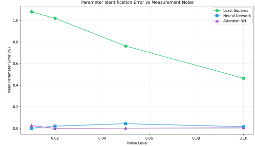
Figure 1. Mean parameter identification error as a function of measurement noise level from a representative experimental run (seed=42). The attention-enhanced neural network maintains consistently low error rates across different noise levels. The pattern shown here is representative of the consistent performance observed across all 5 independent runs (see Table 1 for averaged results).
