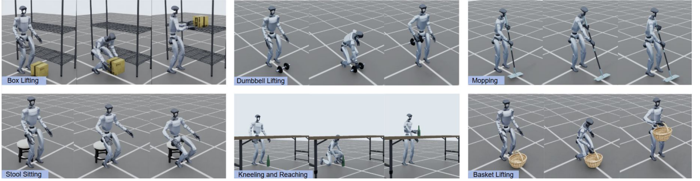
Fig. 3: Synthesized robot-object references. We show box lifting, dumbbell lifting, floor mopping, stool sitting, kneeling and reaching, and basket lifting, all produced by the same pipeline. Each panel contains temporally ordered keyframes from one generated and reconstructed trajectory.
