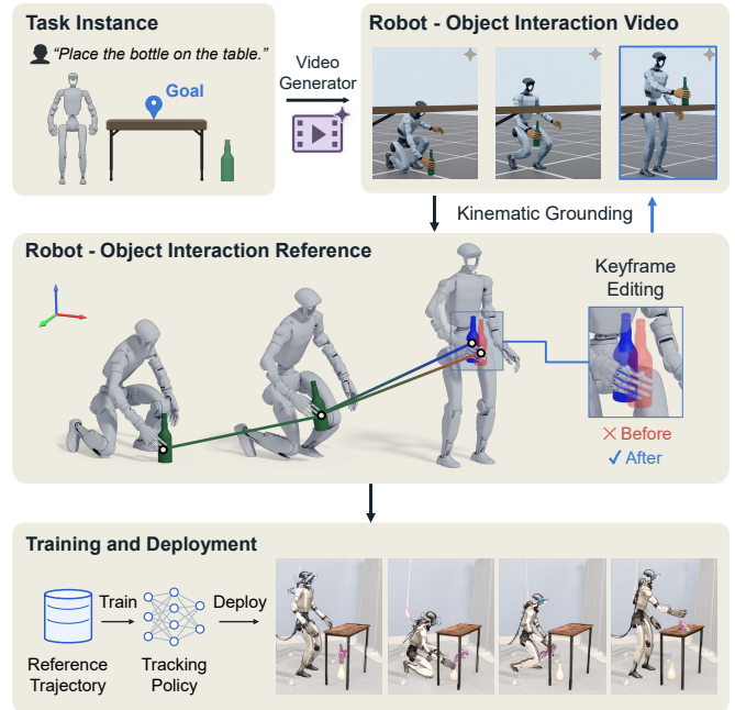
Fig. 1: KinoGen synthesizes and customizes humanoid loco-manipulation references for the target embodiment. A task specification and calibrated simulator render condition robot-video generation; fitting the target robot and object models to the generated video recovers synchronized whole-body, hand, and object trajectories. Editing a robot-object keyframe conditions regeneration of the intervening motion, while constrained reconstruction enforces the correction. The resulting references train tracking policies deployed on a Unitree G1 with dexterous hands.
