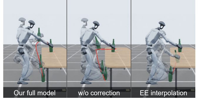
Fig. 6: Metric reference correction. Left: Keyframe-conditioned regeneration proposes a lift-over motion, and constrained reconstruction enforces the target exactly. Middle: Reconstructing the original cue-conditioned video does not reach the prescribed target. Right: Direct end-effector interpolation reaches the target but moves the hand and bottle through the table.
