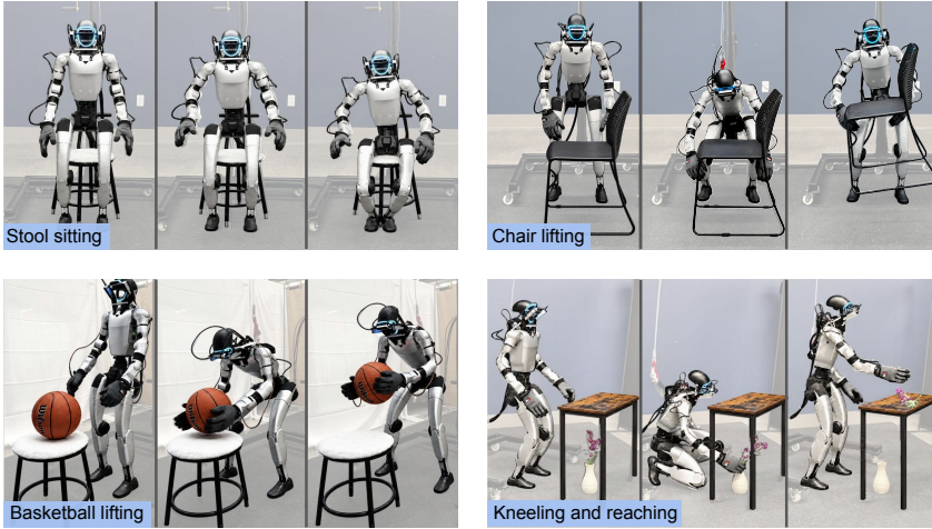
Fig. 4: Hardware deployment of reconstructed references. Tracking policies execute four KinoGen references on a Unitree G1: stool sitting, chair lifting, basketball lifting, and kneeling and reaching. Frames within each panel progress from left to right and show one hardware rollout.
