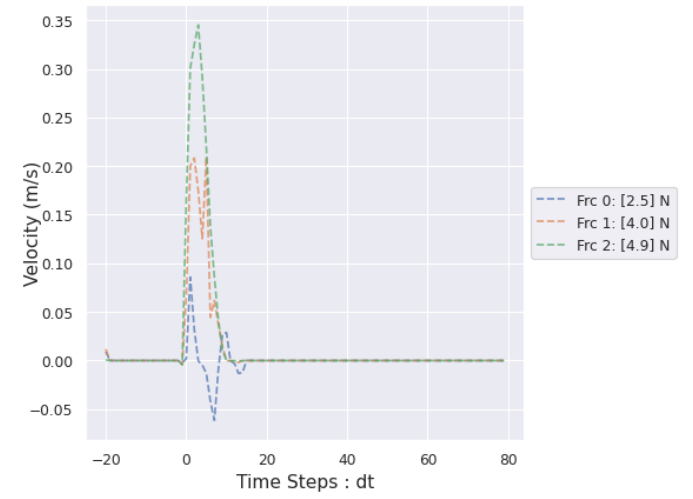
Velocity Trajectories - Lift Weight - Weight value - 3.2N (320gms)
