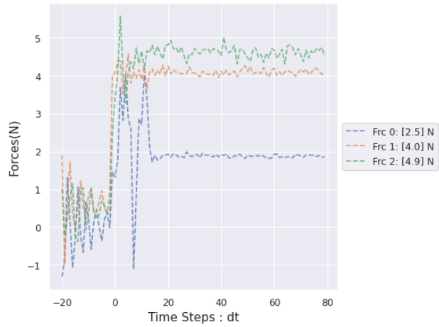
Force Trajectories - Lift Weight - Z - Axis Weight value - 3.2N (320gms)
