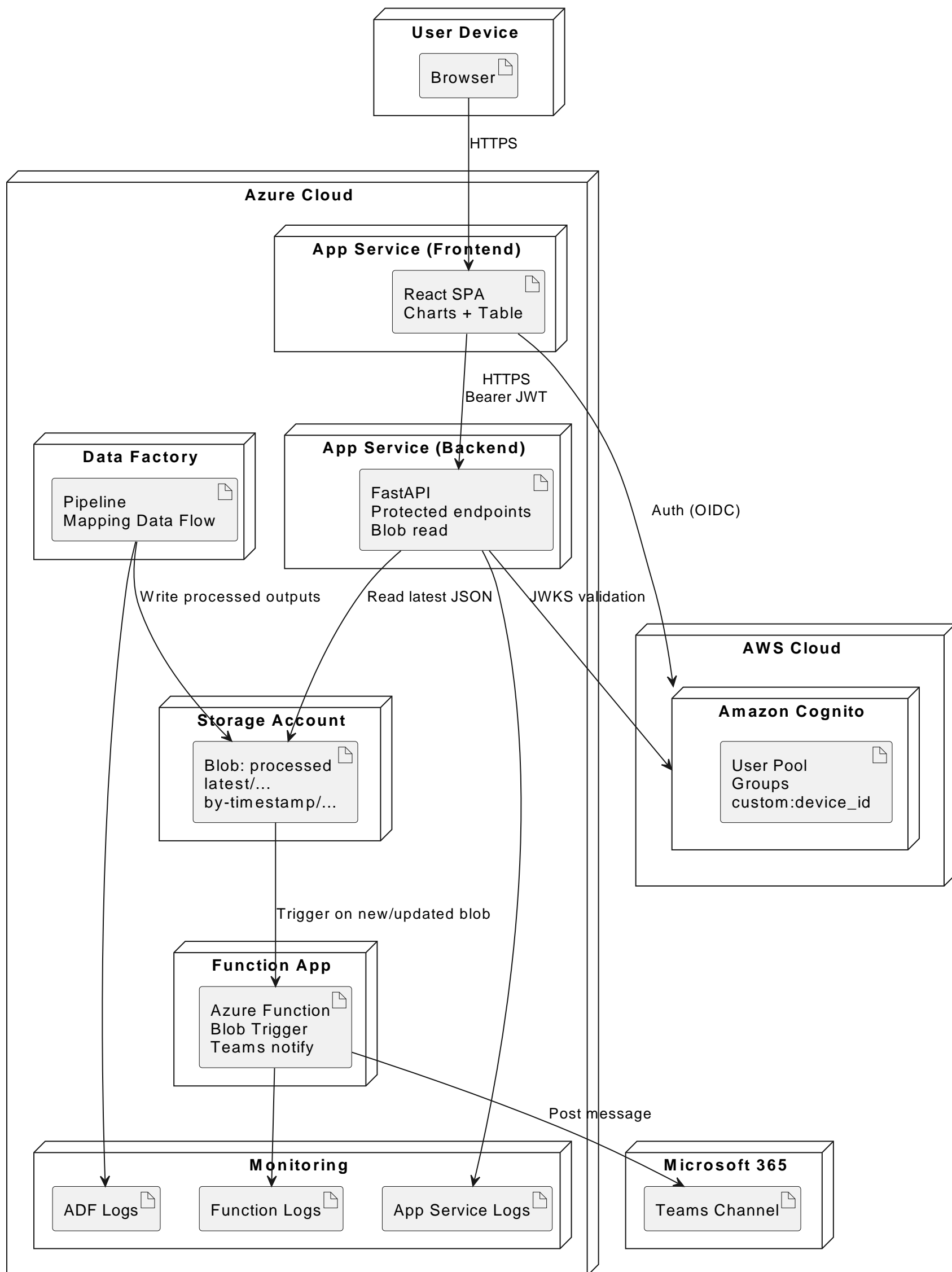
Final - UML Deployment Diagram (End-to-End)
