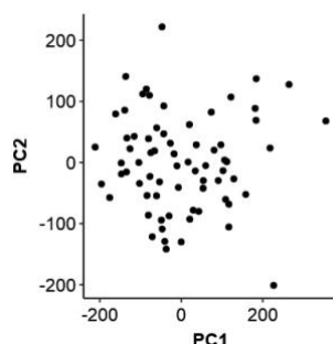
Outlier detection
