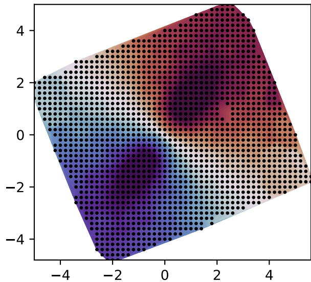
Symmetrized
