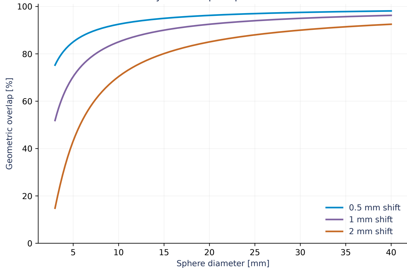
Synthetic equal-sphere model
