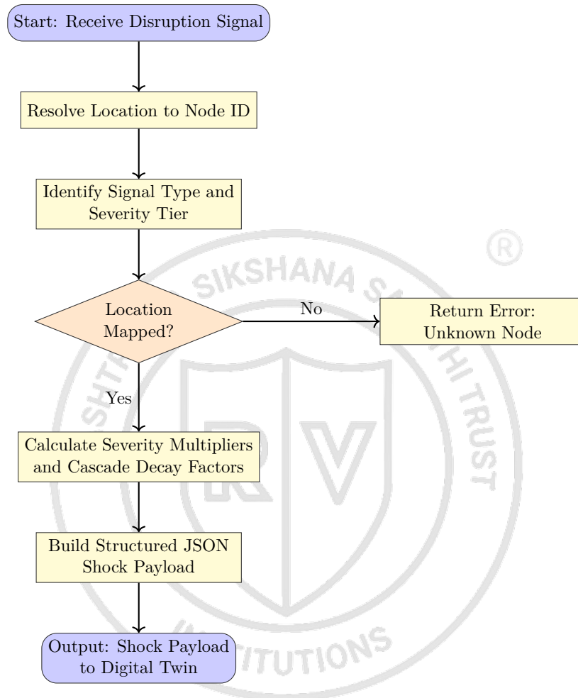
Figure 5.3: Flowchart of Friction Sentry Module
