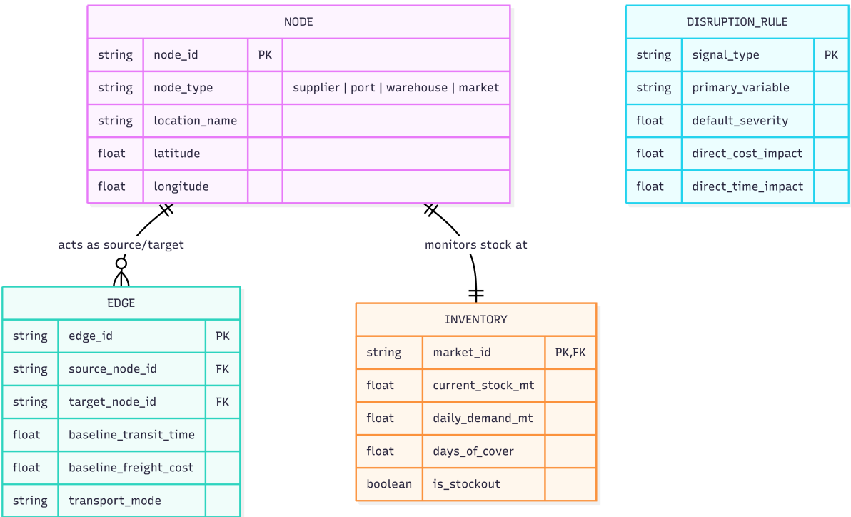
Figure 5.7: Entity-Relationship Diagram for Logistics Digital Twin
