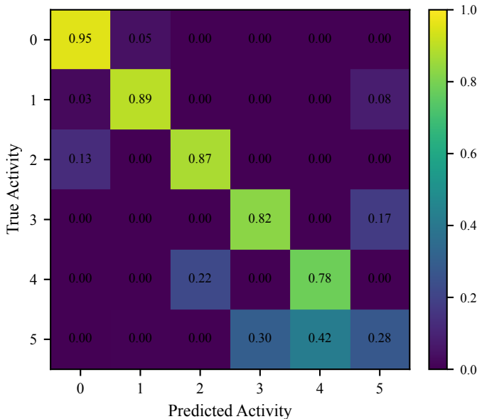
Normalized Test Confusion Matrix
