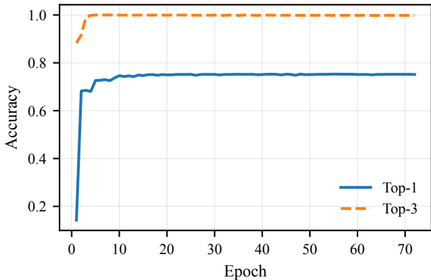
Validation Top-k Accuracy
